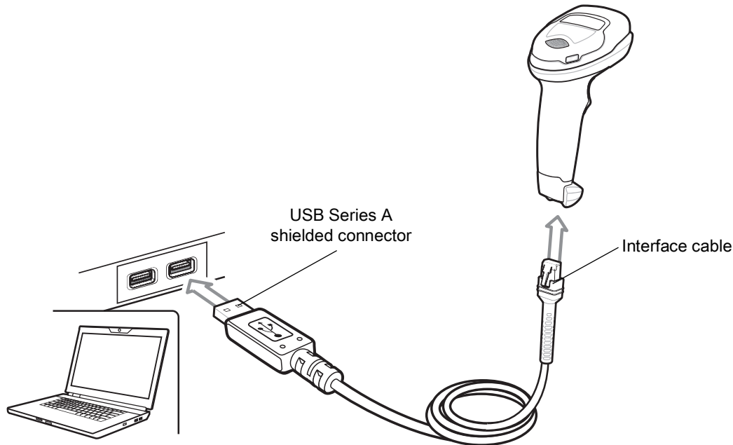
Figure 16 USB Connection
