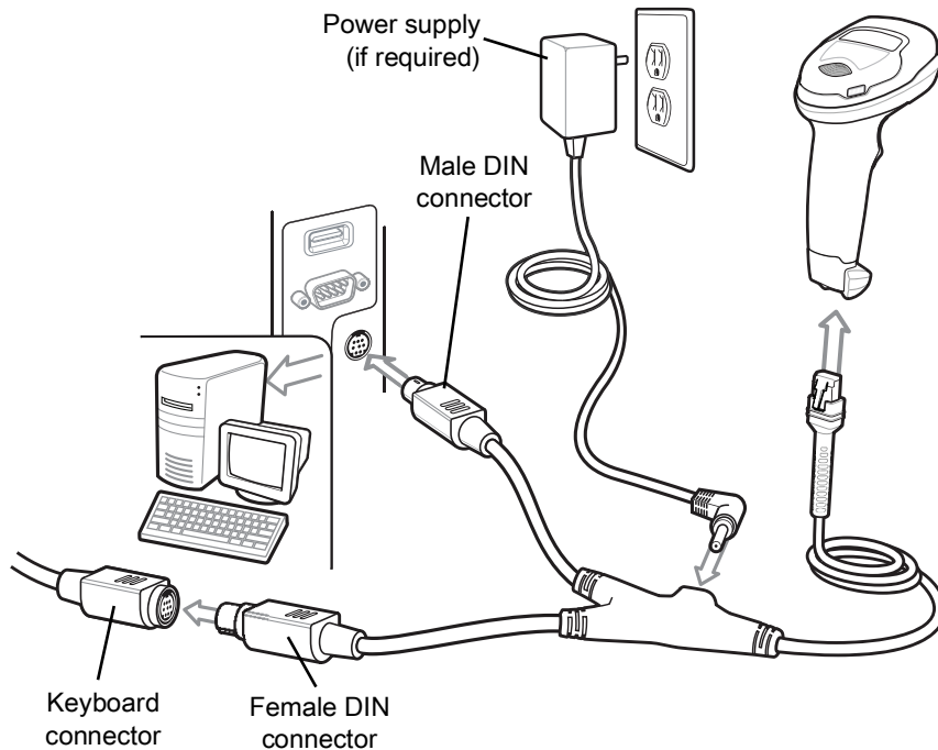
Figure 19 Keyboard Wedge Connection
