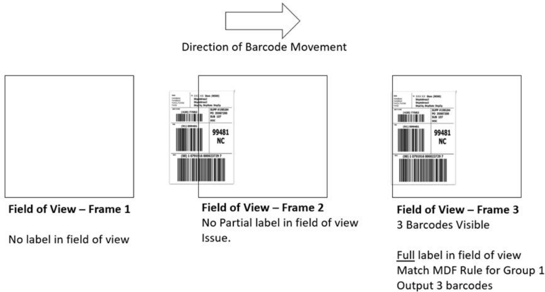
Figure 5 Scanning Label in a Vertical Orientation
