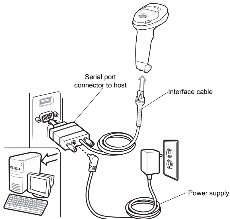
Figure 17 RS-232 Connection
