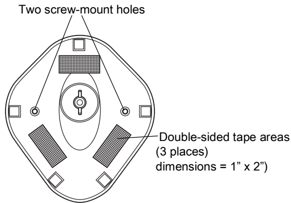
Figure 8 Mounting the Stand
