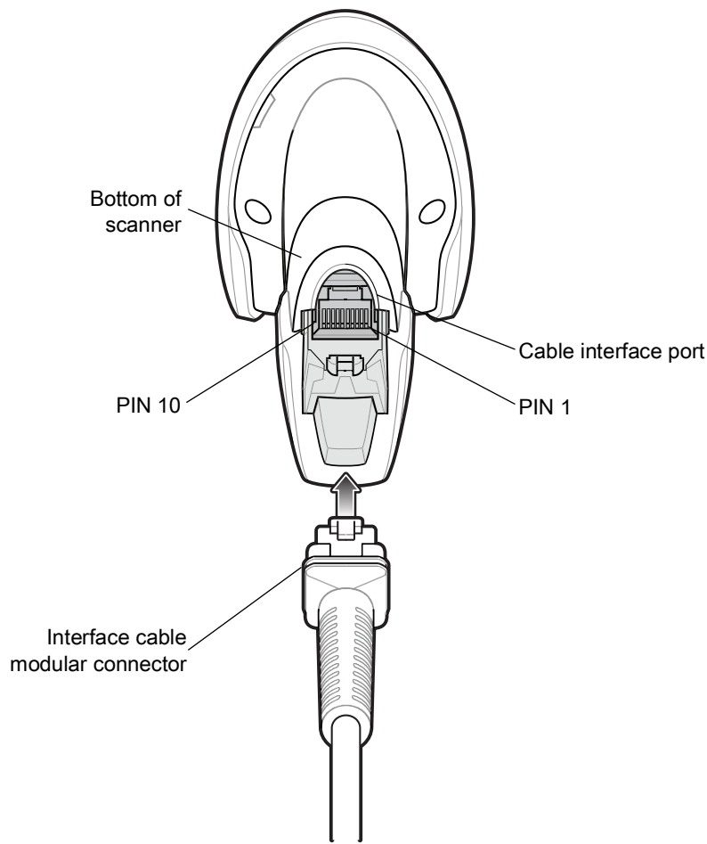
Figure 15 Imaging Scanner Cable Pinouts
