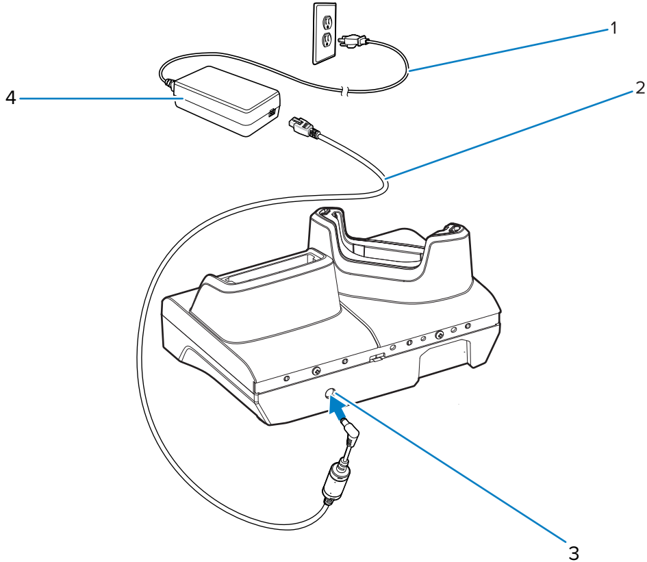
Figure 30 1-Slot Cradle with Spare Battery Slot Setup
