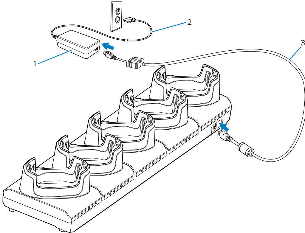
Figure 33 5-Slot Charge Only Cradle Setup
