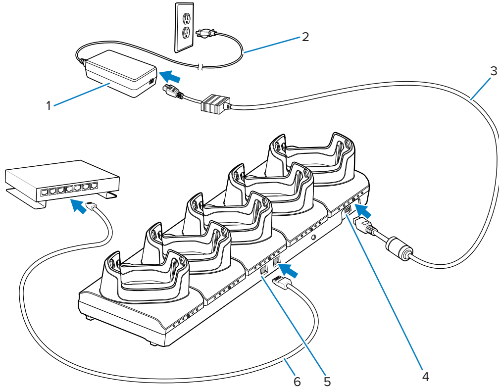
Figure 35 5-Slot Ethernet Cradle Setup
