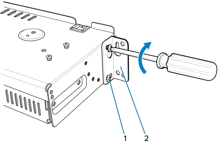
Figure 42 Flange Horizontal Position (5-Slot Cradles)
