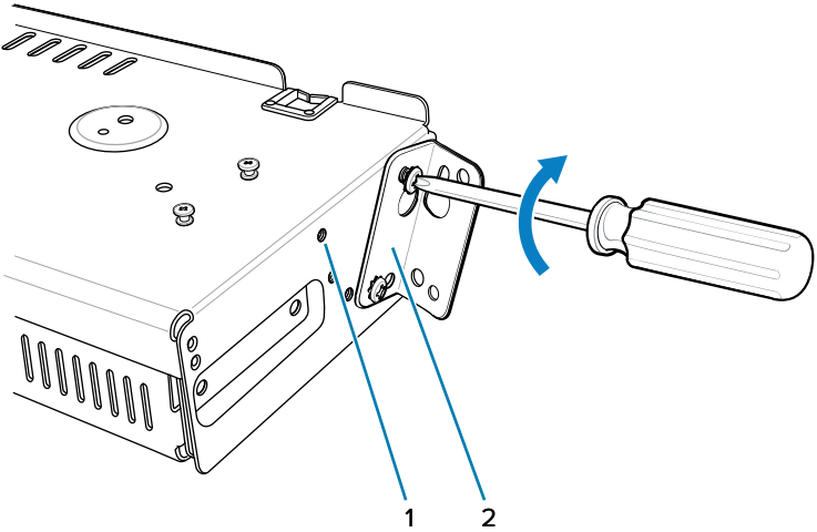
Figure 43 Flange 25° Position (4-Slot Battery Chargers)
